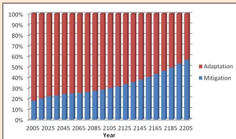
Figure 4: Temporal Investment (percentage) of Adaptation and Mitigation in the Model with Both Adaptation and Mitigation Investment Allowed
